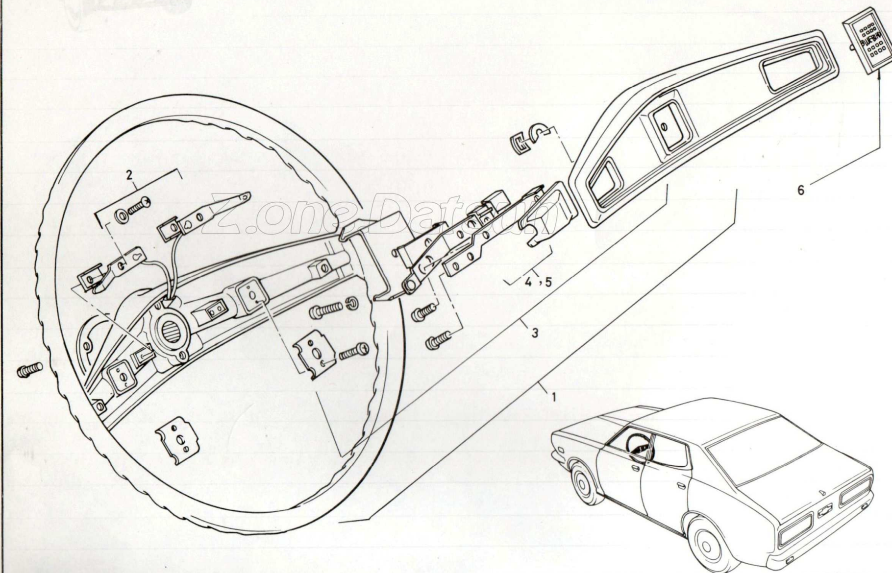
Assy-wheel, steering
